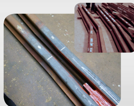
Schienenknick biegen Rail kink bending
